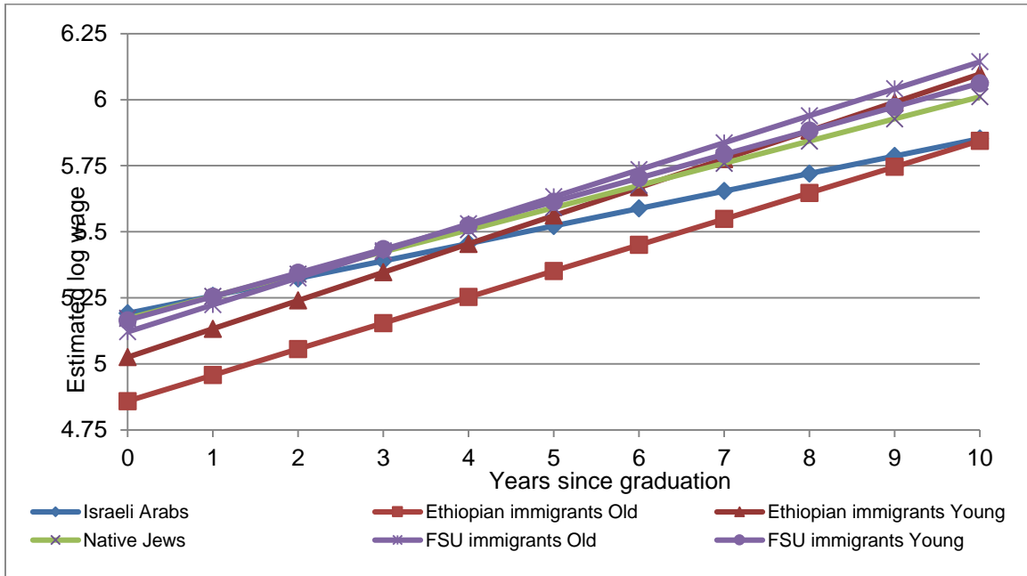
Figure 3e: Estimated log wage by ethnic group, age on arrival and years since graduation allowing the return on experience to vary with psychometric score - Men only
