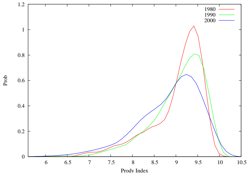
Figure 1: PRODY index, kernel densities in 1980, 1990 and 2000.
