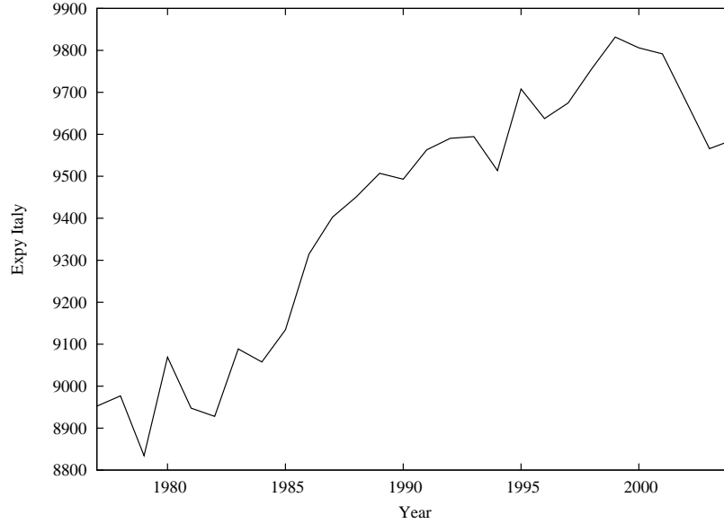
Figure 5: EXPY index for Italy, 1977-2004
