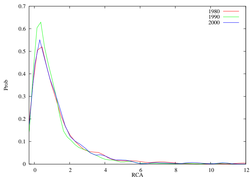
Figure 3: RCA of Italy, kernel densities over time
